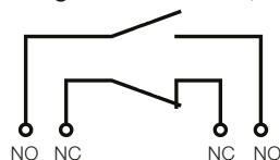
Diagrama - FSW 100, 160, 250, 400
